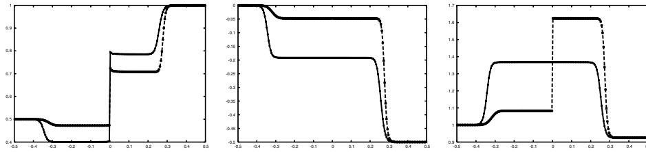
FIGURE 7. \tau, v, p in the transmission of \mathbf{u} = (\tau, v, e) vs. \mathbf{v} = (\tau, v, p) the for Euler system: Discontinuity of \tau – Continuity of v – Continuity of p for \mathbf{v} / Discontinuity of p for \mathbf{u}
