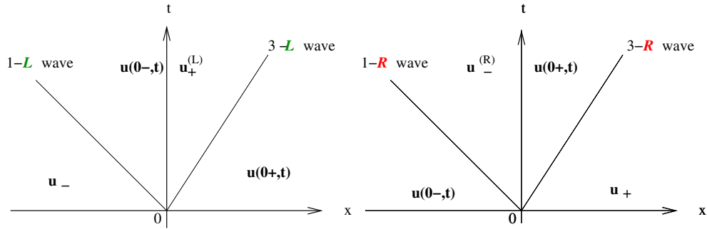
FIGURE 5. Coupling conditions (5) for the Euler system: \mathbf{u}(0-, t) \in \mathcal{O}_L(\mathbf{u}(0+, t)) (left), \mathbf{u}(0+, t) \in \mathcal{O}_R(\mathbf{u}(0-, t)) (right)
