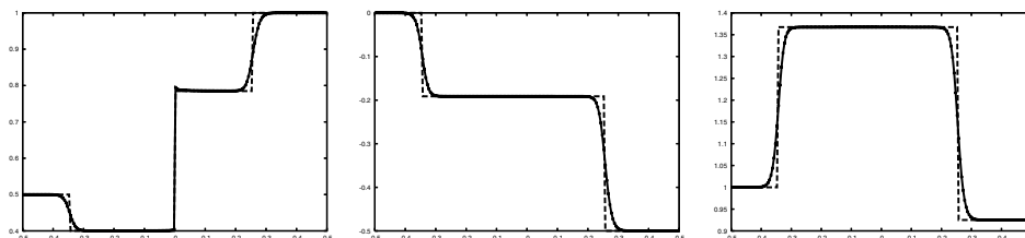
FIGURE 4. \tau, v, p for the coupled Riemann problem for the Euler system with transmission of \mathbf{v} = (\tau, v, p) : discontinuity of \tau , continuity of v, p at x = 0
