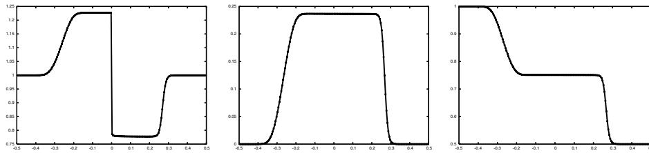
FIGURE 9. \tau, v, p for the transmission of \mathbf{v} = (v, p) , p -system in x < 0 and Euler then system in x > 0
