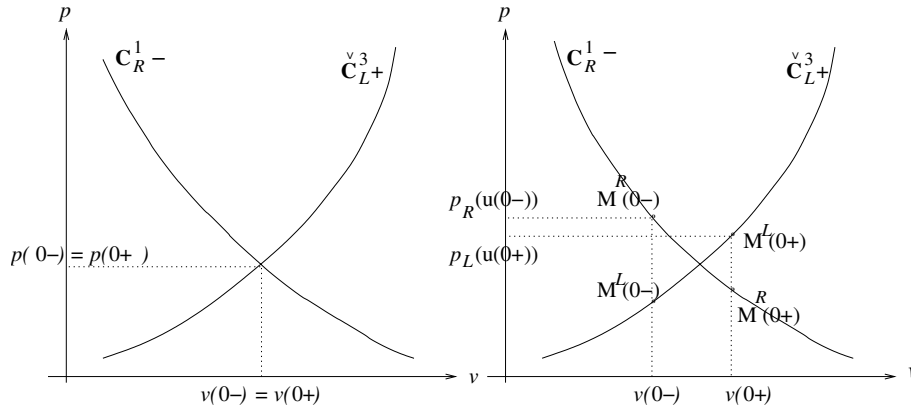
FIGURE 6. Projection of the wave curves: transmission of \mathbf{v} (left)–transmission of \mathbf{u} (right), with \mathbf{C}_R^1- = \mathbf{C}_R^1(\mathbf{v}(0-)) , \check{\mathbf{C}}_L^3+ = \check{\mathbf{C}}_L^3(\mathbf{v}(0+))
