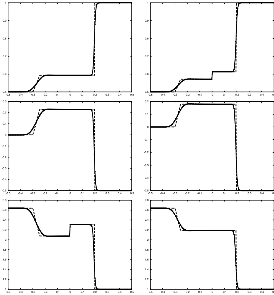
FIGURE 3. \tau, v, p in the transmission of \mathbf{u} = (\tau, v) left / vs. \mathbf{v} = (v, p) right for the coupled p -system: continuity of (\tau, v) left / vs. continuity of (v, p) right (numerical and exact solution)
