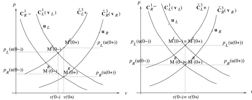
FIGURE 8. Coupled Riemann problem, projection of the wave curves: general case (left), special case (right), with C_R^{1-} = C_R^1(\mathbf{v}(0-)) , \check{C}_L^3+ = \check{C}_L^3(\mathbf{v}(0+))
