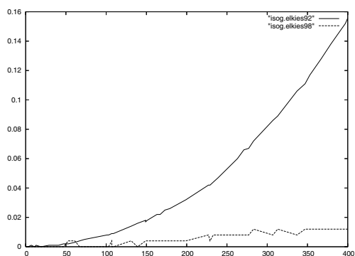
FIGURE 2. Elkies1992 vs. Elkies1998.
