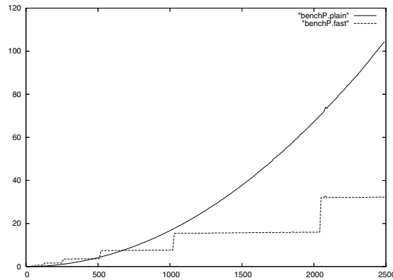
FIGURE 1. Timings for computing \varphi on E : y^2 = x^3 + 4589x + 91128 over \mathbb{F}_{10^{2004}+4683}
