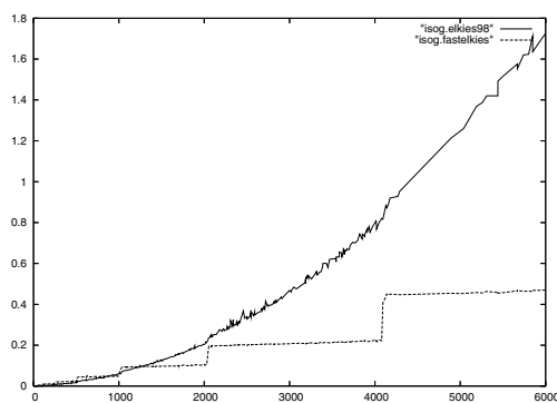
FIGURE 3. Elkies1998 vs. fastElkies.
