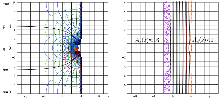
FIGURE 4. Left: Function f = F_{4,5}(z) in the x+iy plane; levels p = \Re(f)=\text{const} and levels q = \Im(f)=\text{const} are shown with thick lines for integer values of p and q . Right: Function f = A_4(z) by (4.13) in the x+iy plane; levels f = 1, 4, 8, 12, 16 are shown with thick lines.
