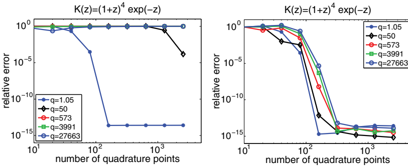
FIGURE 3. Convergence rates for different values of q . Left: With the simple parametrization of \mathcal{C}_M given by M(1 + \exp(i\theta)) , \theta \in [0, 2\pi) . Right: With the parametrization in Definition 7.
