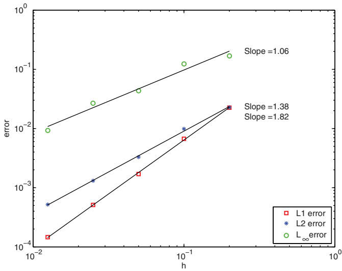
FIGURE 4. Example 2, Q^2 elements.
