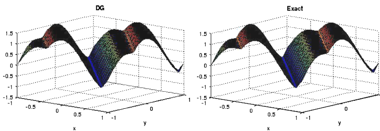
FIGURE 5. Example 2 at time t = 0.5 , numerical (left) and exact (right) data, using Q^2 elements with N_x = 20 mesh cells
