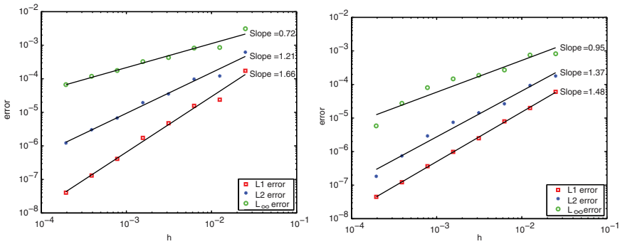
FIGURE 3. Example 1, SLDG scheme, with P^2 elements. Left: \Delta t = h/2 , Right: \Delta t = Ch^{3/5} .
