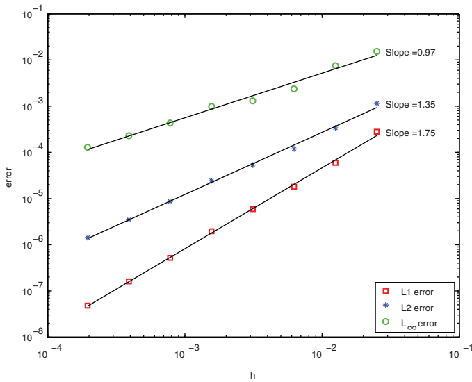
FIGURE 2. Example 1, RKDG scheme with P^2 elements.
