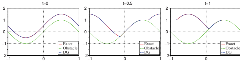
FIGURE 1. Example 1, RKDG scheme, times t = 0, t = 0.5 and t = 1 , using P^2 elements with N_x = 20 mesh cells (obstacle: green dotted line).
