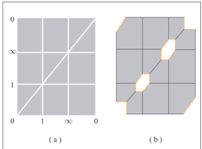
Figure 11. \mathcal{M}_0^5(\mathbb{R}) before and after compactification.
