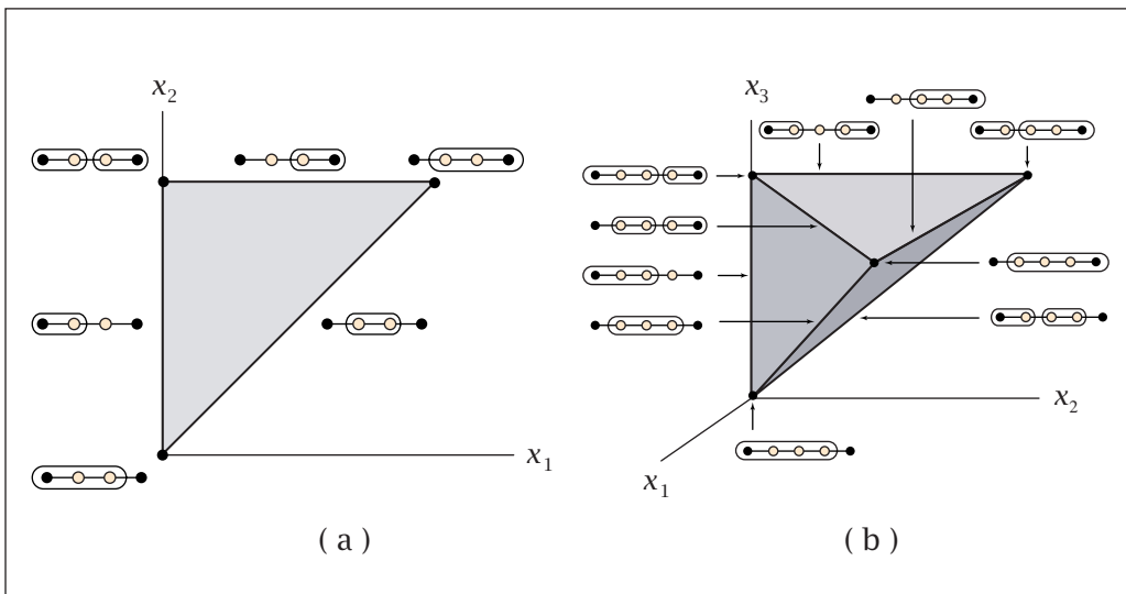
Figure 1. Labeling of vertices and edges of \Delta_2 and \Delta_3 .
