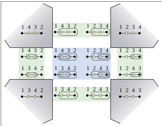
Figure 10. A local tiling of PV^2_{\#} displaying twisting.
