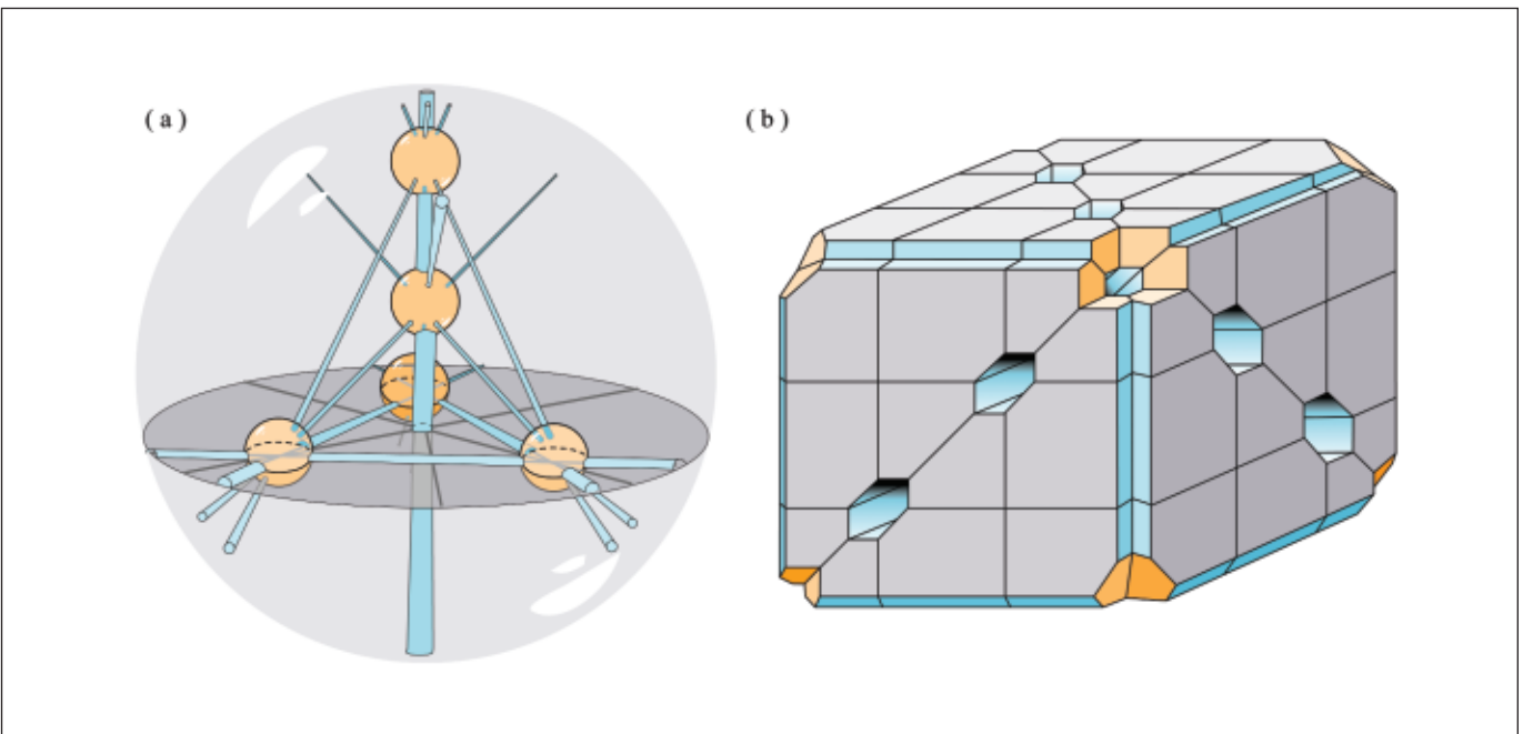
Figure 12. Iterated blowups of (a) \mathbb{R}P^3 to PV^3_{\#} and (b) T^3 to \overline{\mathcal{M}}_0^6(\mathbb{R}) are both homeomorphic with a tiling by 60 associahedra.
