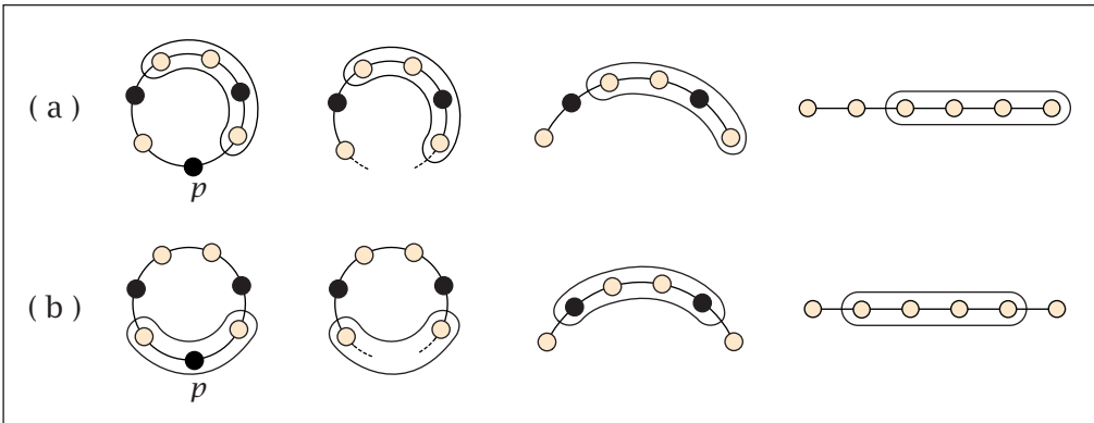
Figure 6. Bijection from \mathcal{B}(n) to \mathcal{A}(n) .
