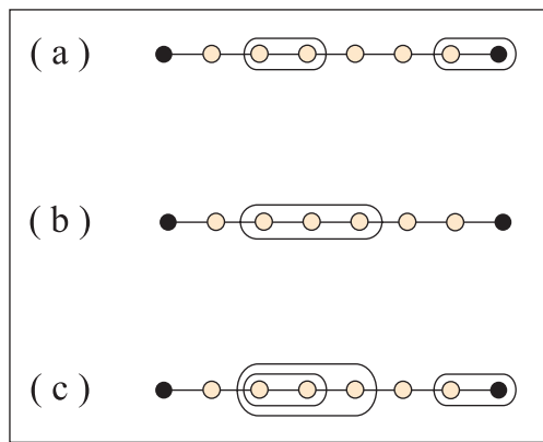
Figure 3. Compatibility of bracketings.
