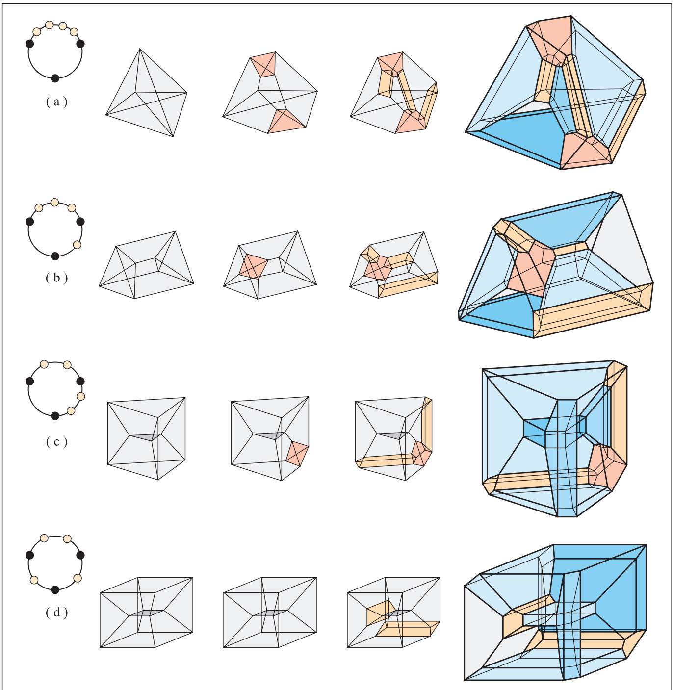
Figure 13. Schlegel diagrams of the iterated truncations of 4-polytopes resulting in K_6 .
