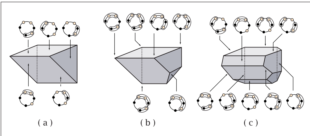
Figure 7. Truncation and labeling of \Delta_2 \times \Delta_1 .
