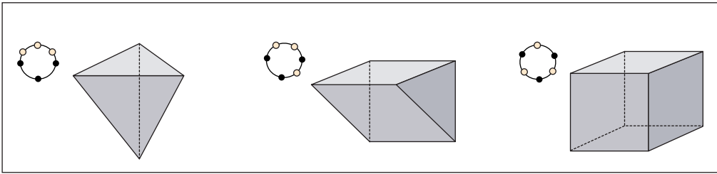
Figure 5. Three types of simplicial products with three particles.
