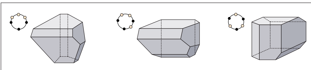
Figure 8. Iterated truncations of polytopes resulting in K_5 .
