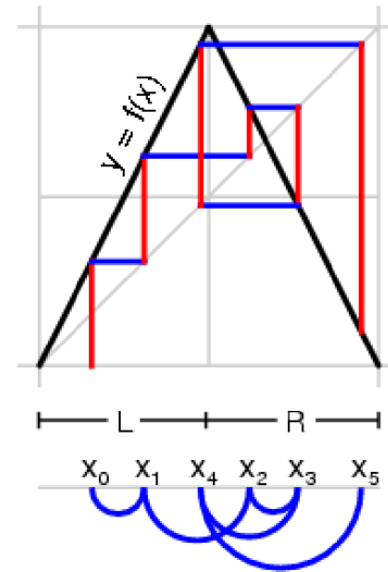
Figure 2. Iterations of the function f(x) simulate the random behavior of the previous figure. In this case the initial value x_0 produces LLRRLR...
