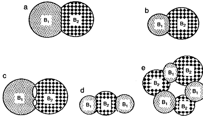
FIGURE 1. Foisy et al. [F] proved that the standard double bubble (a, b) is the least-perimeter way to enclose and separate two regions of prescribed areas in the plane, rather than any other crazy alternative.
