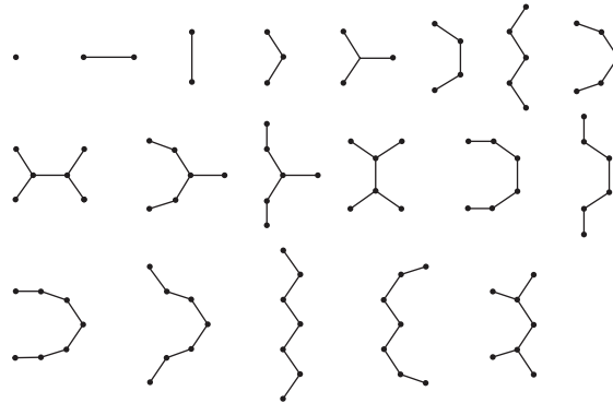
FIGURE 1. Hubbard trees for degrees 2 \leq n \leq 8 . The real line is the horizontal line of symmetry for each tree, and the induced mapping on the trees is complex conjugation. All angles are multiples of 2\pi/3 .
