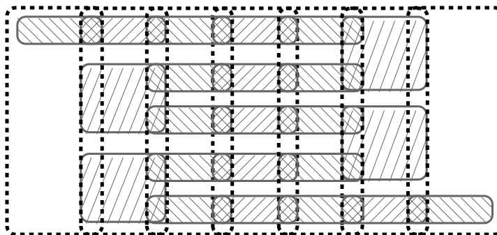
FIGURE 1. Proper 5-fold.
