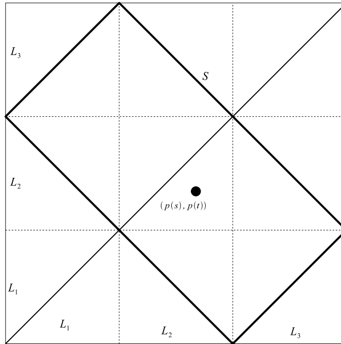
FIGURE 2. The set G .
