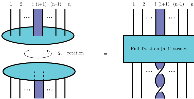
FIGURE 1. Full twist on n strands, with two consecutive strands grouped together as one strand.
