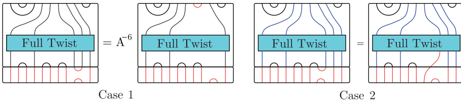
FIGURE 3. Two cases for Lemma 2.2
