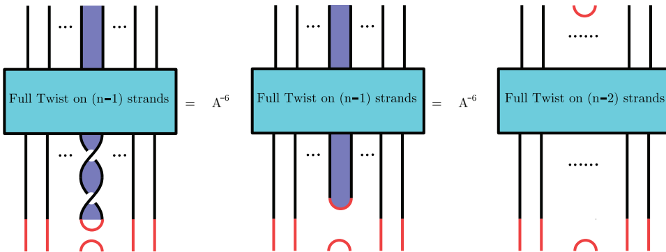
FIGURE 2. \Delta_n^2 e_i = A^{-6} E_i
