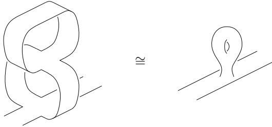
FIGURE 7. Connected sum with a torus
