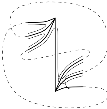
FIGURE 3. Chain of circles
