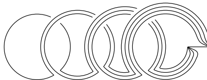
FIGURE 2. Iterated images of an interval
