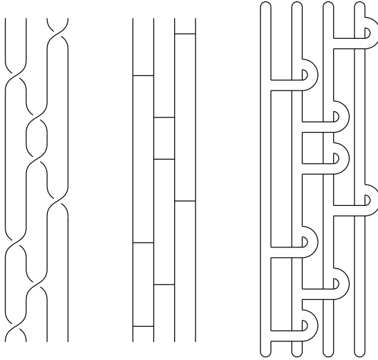
FIGURE 4. Positive braid, brick diagram and fibre surface
