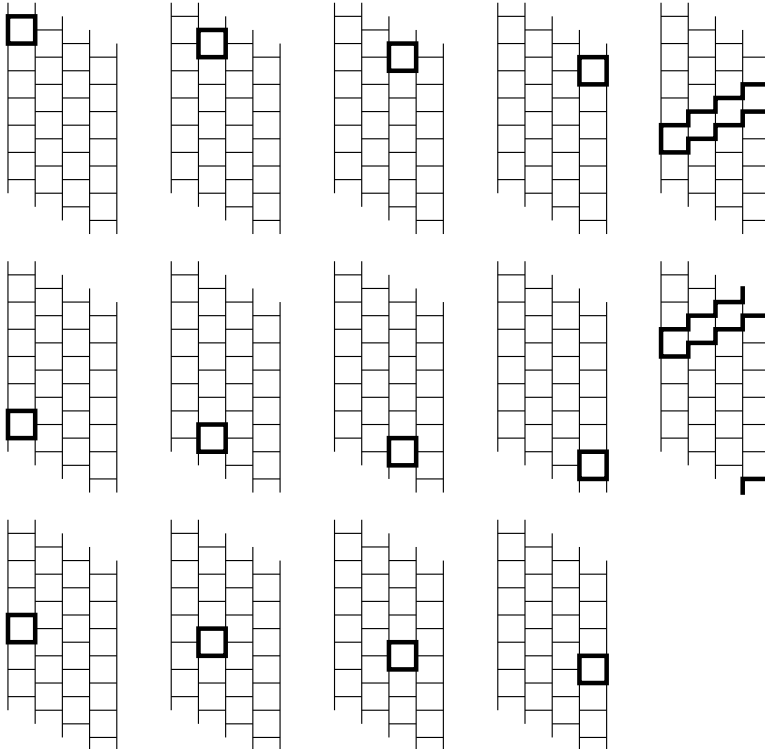
FIGURE 11. From R to \phi^{13}(R)
