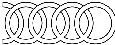
FIGURE 1. Iterated Hopf plumbing
