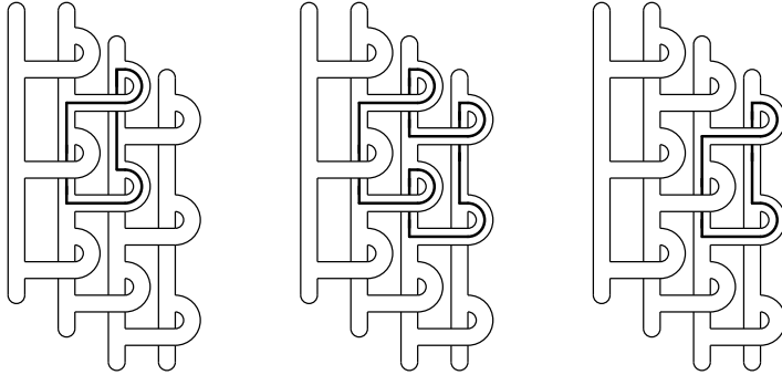
FIGURE 8. From \phi(R) to \phi^2(R)
