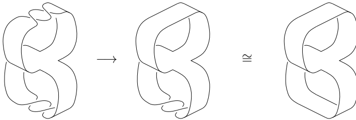
FIGURE 6. A ribbon twist
