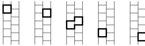
FIGURE 10. From R to \phi^4(R)
