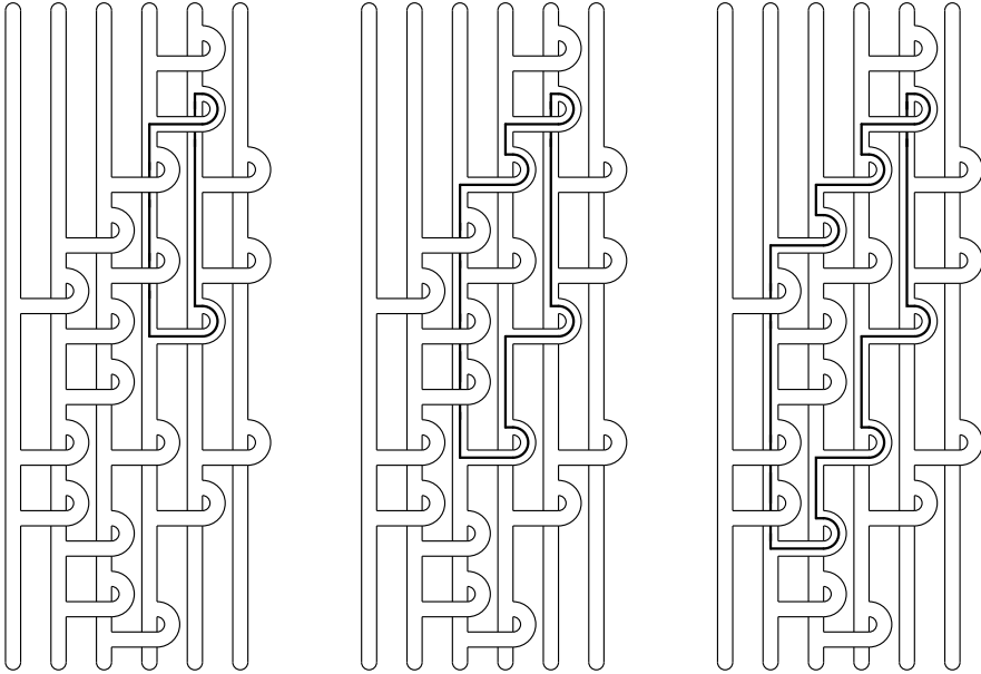
FIGURE 5. From \phi_4\phi_5(R) to \phi_2\phi_3\phi_4\phi_5(R)
