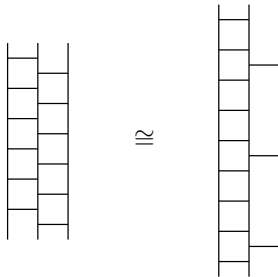
FIGURE 9. \Sigma(3, 6) contains \Sigma(2, 9)
