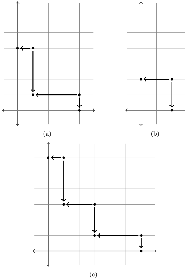
FIGURE 1. (a), CFK^\infty(T_{2,3;2,5}) . (b), the relevant summand of CFK^\infty(T_{4,5}\# - T_{2,3;2,5}) from the statement of Lemma 2.1. (c), CFK^\infty(T_{4,5}) . More precisely, CFK^\infty is generated over \mathbb{F}[U, U^{-1}] by the generators depicted.
