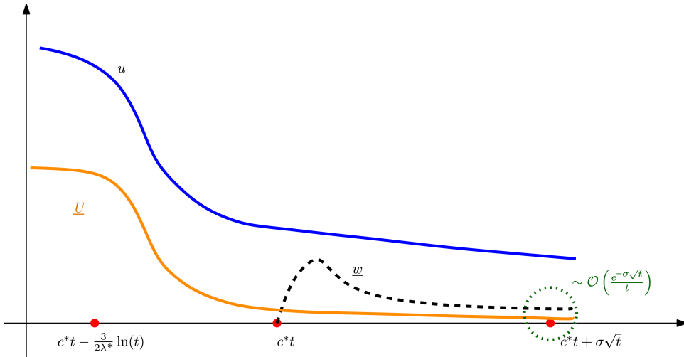
FIG. 2. A sketch of the sub-solution \underline{U} , the solution u of the Fisher-KPP problem, and of the solution of the linearized problem with the Dirichlet boundary condition at x = c^*t .
