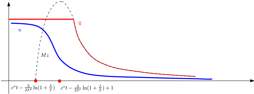
FIG. 1. A sketch of the solution u and the super-solution \bar{u} .
