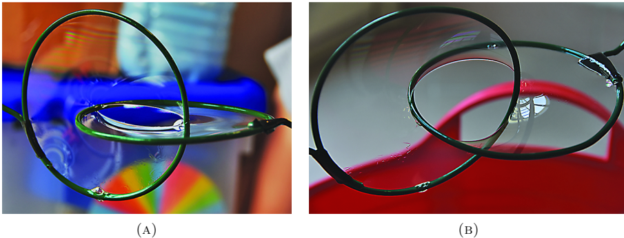
FIG. 3. Results obtained by our configuration with two fixed linked rigid metallic wires.
