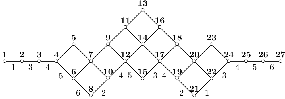
FIGURE 1. (E_6, \varpi_1) .
