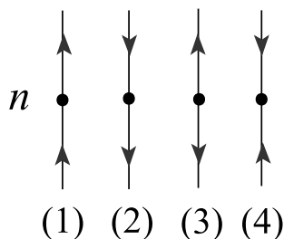
FIGURE 3. The vertex representation of the matrix entries of the L -operator.
