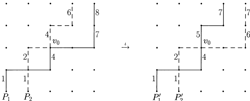
FIGURE 5. The involution of Theorem 4.1
