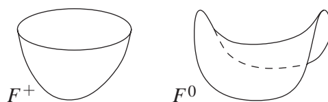
FIGURE 15. Types of critical points in a 2-cell
