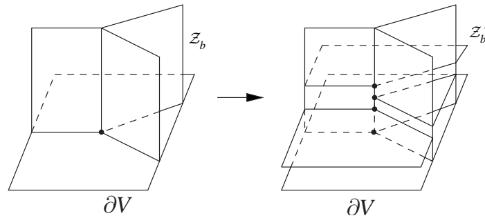
FIGURE 13. Subdividing 3-cells of Z_b
