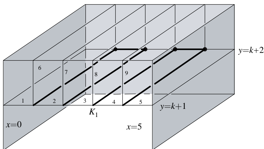
FIGURE 7. Realization of the caps of b
