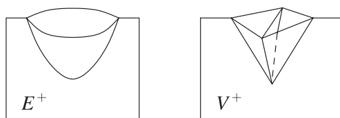
FIGURE 14. Types of critical points in \mathcal{C}^1
