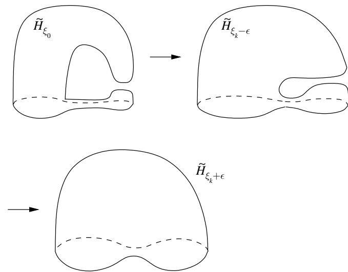
FIGURE 17. The moves of \tilde{H}
