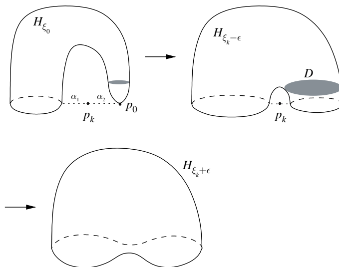
FIGURE 16. The moves of H
