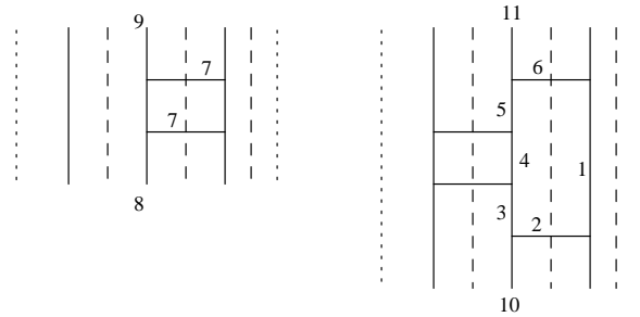
FIGURE 10. \partial V in the cups of b
