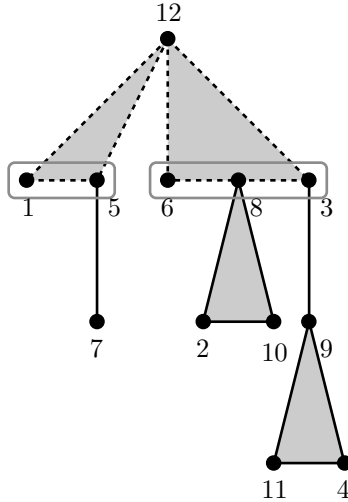
FIGURE 2. A rooted hypertree on [12] with its associated planted hyperforest on [11] . One can pass from the hyperforest back to the hypertree using the partition of \{1, 3, 5, 6, 8\} indicated by the lightly colored boxes.
