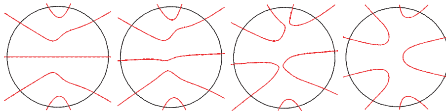
FIGURE 1. The curves C_\theta(f) , where f(z) is the quintic z^5 + 6z^3 + 3z^2 + 5z - 2 , and \theta = 0, \frac{\pi}{12}, \frac{\pi}{6}, \frac{\pi}{2} respectively.
