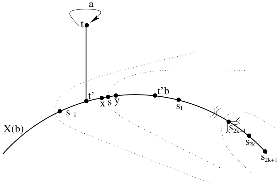
FIGURE 1. Mining out randomness
