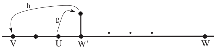
FIGURE 2. Transitive action on the even vertices
