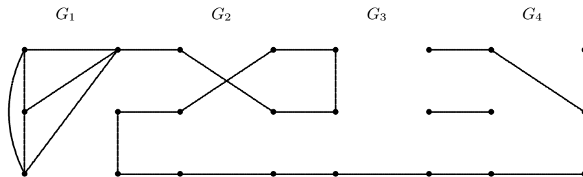
FIGURE 2. A graph G_{\mathcal{P}} , with S = [3] and m = 4 .
