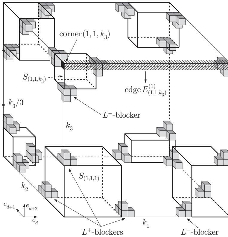
FIGURE 1. The set [m_1] \times \cdots \times [m_{d-1}] \times [k_1] \times \cdots \times [k_{\ell+1}] , with examples of blockers and edges. Observe that the d - 1 first dimensions are not depicted: each ‘unit’ square is a set \mathcal{M}_{\mathbf{x}} .
