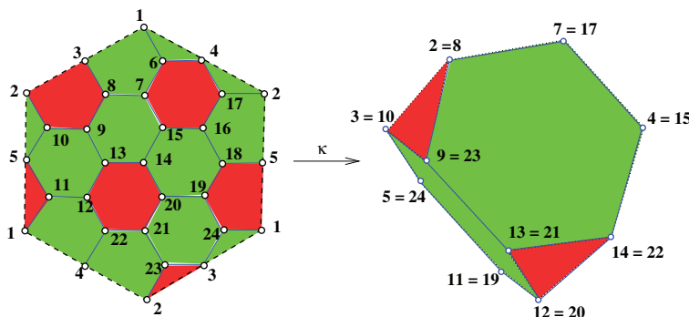
FIGURE 3. The toroid \{6, 3\}_{(2,2)} covers the truncated tetrahedron.
