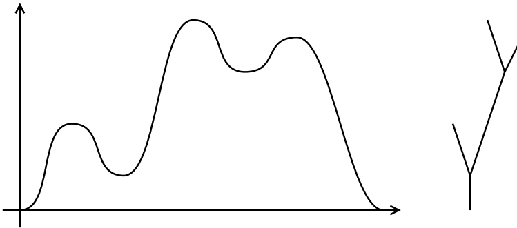
FIGURE 6. An excursion and associated real tree.
