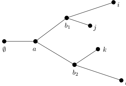
FIGURE 8. A possible configuration of i, j, k, l .
