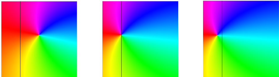
FIGURE 3. Phase plots of 1 - f(\gamma w) for \alpha = 30, 60, 80 . The black line indicates the set \{z \in \mathbb{C} : \Re z = 1/2\} . The region of the plot is \{z \in \mathbb{C} : \Re z \in [0, 2] \text{ and } \Im z \in [8, 10]\} .
