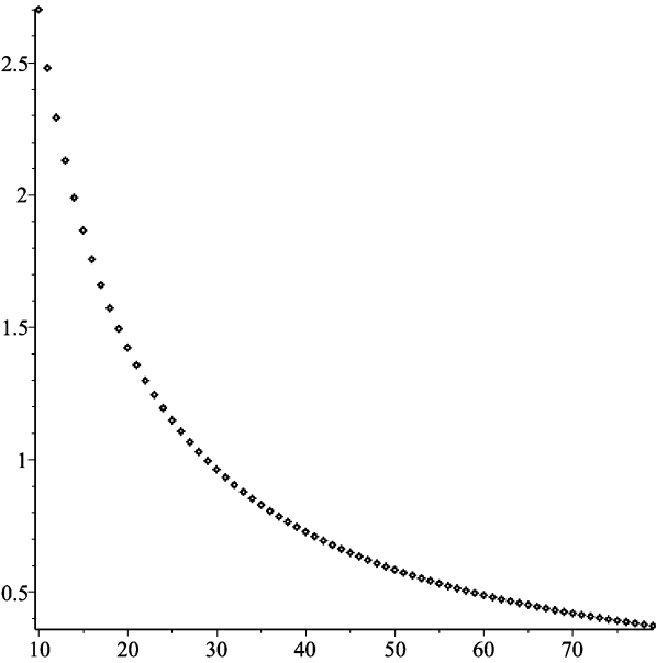
FIGURE 4. Plot of the real part of the root of 1 - f(\gamma w) in \Re z > 0 closest to the imaginary axis against \alpha .
