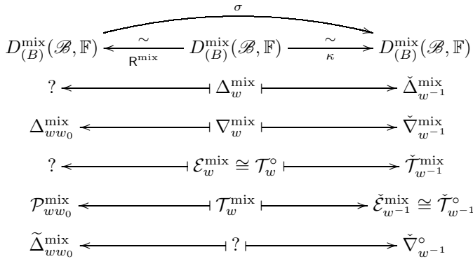
FIGURE 1. Behavior of various objects under the equivalence \sigma .
