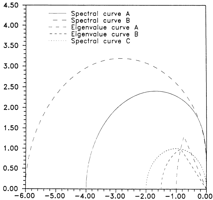
FIGURE 1 Comparison of spectral and eigenvalue curves
