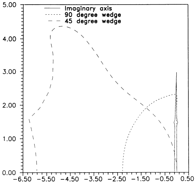
FIGURE 2d Stability regions for k = 2 , m = 3 , p = 2 schemes
