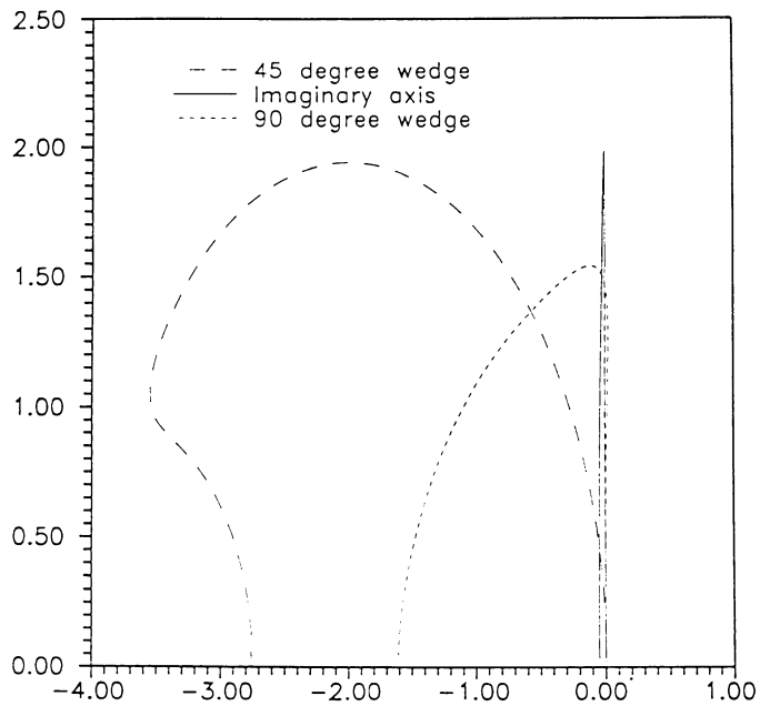
FIGURE 2b Stability regions for k = 2 , m = 2 , p = 2 schemes
