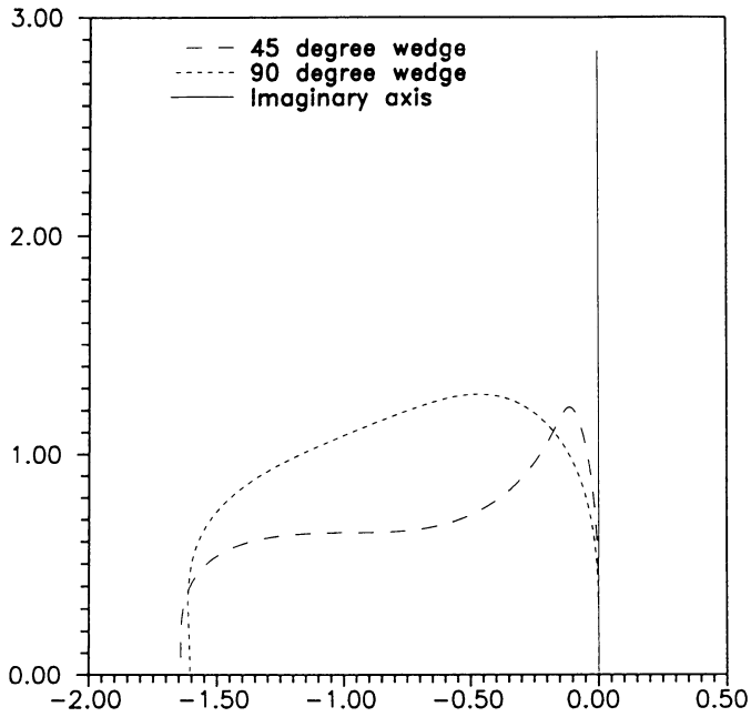
FIGURE 2c Stability regions for k = 2 , m = 3 , p = 3 schemes
