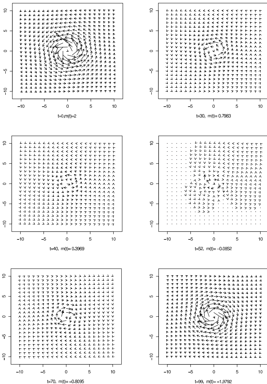
FIGURE 3. \varepsilon = 10^{-4} , \nu = 5 \times 10^{-7} , n = 1000 , T = 100 , \Delta t = 1 , p = \frac{1}{3} , sign(\gamma) = -1 .
