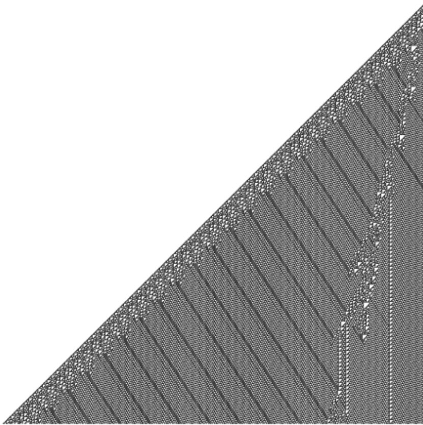
Figure 2. The first 750 updates for rule 110.
