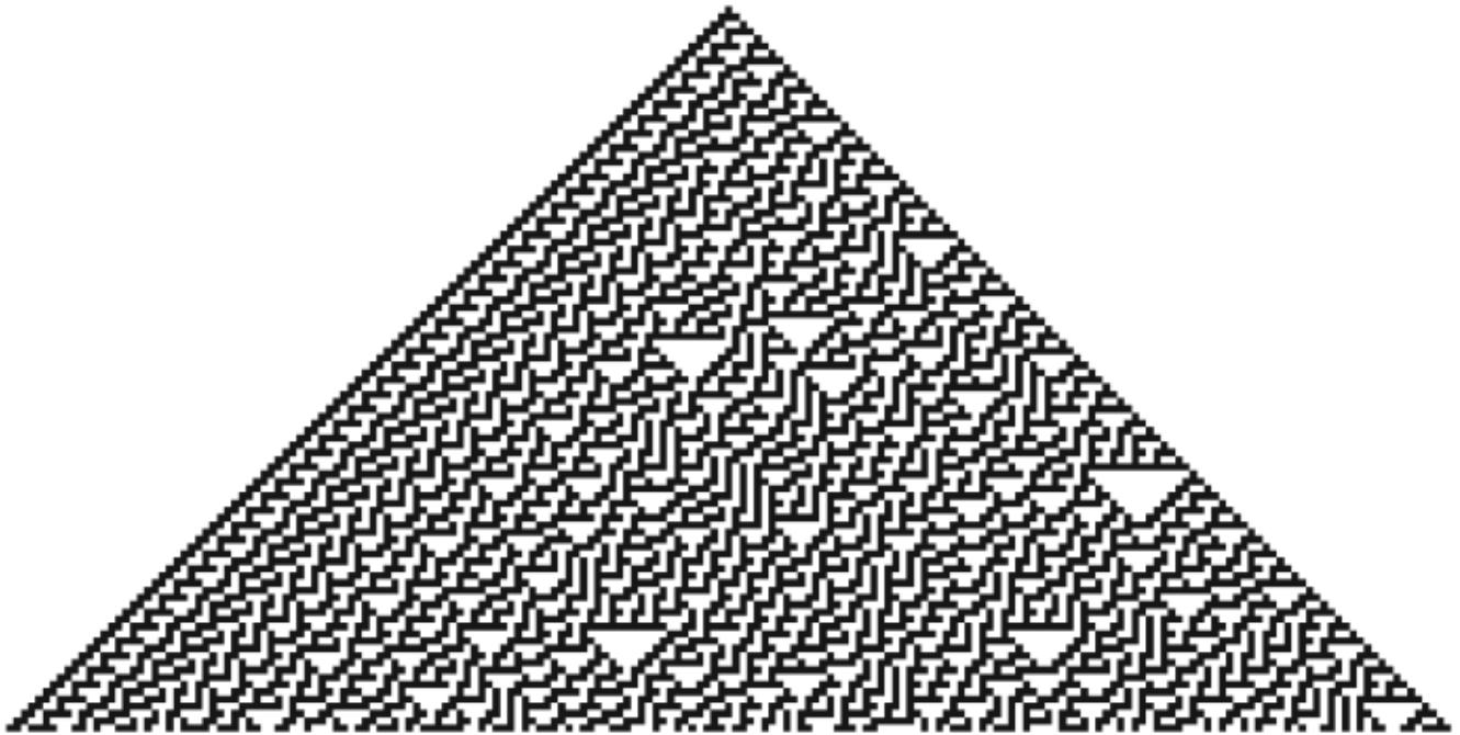
Figure 1. The first 100 updates for Rule 30.
