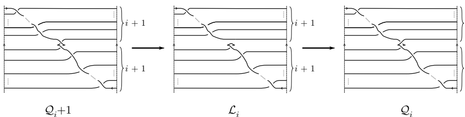
FIGURE 7. The first arrow indicates a cobordism between \mathcal{Q}_{i+1}(K) and L_i(K) and the second arrow indicates a cobordism between L_i(K) and \mathcal{Q}_i(K) . Note that the right panel is the middle panel of Figure 5
