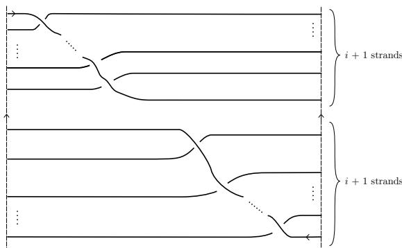
FIGURE 6. A Legendrian diagram \mathcal{L}_i for the pattern L_i . We compute that \text{tb}(\mathcal{L}_i) = 2i , \text{rot}(\mathcal{L}_i) = 0 and w(\mathcal{L}_i) = 0 .
