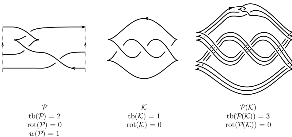
FIGURE 1. The Legendrian satellite operation
