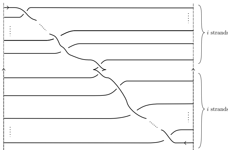
FIGURE 4. A Legendrian diagram \mathcal{Q}_i for the pattern Q_i . We compute that \text{tb}(\mathcal{Q}_i) = 2i - 1 , \text{rot}(\mathcal{Q}_i) = 0 and w(\mathcal{Q}_i) = 0 .
