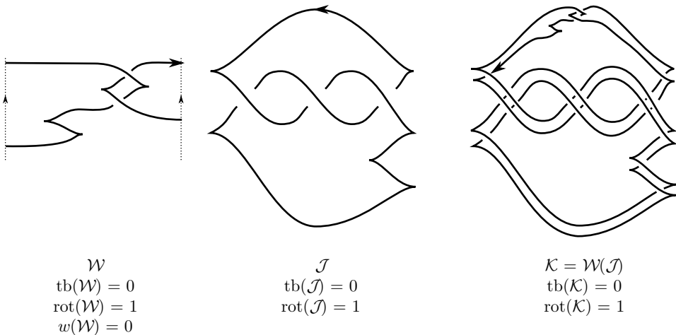
FIGURE 2. Constructing the knots \mathcal{K} .
