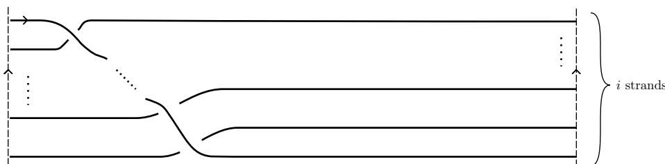
FIGURE 3. A Legendrian diagram \mathcal{P}_i for the pattern P_i . We compute that \text{tb}(\mathcal{P}_i) = i - 1 , \text{rot}(\mathcal{P}_i) = 0 and w(\mathcal{P}_i) = i .
