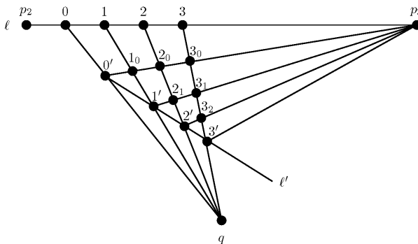
FIGURE 1. The plane P_* .
