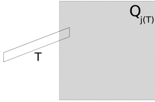
FIGURE 3. A parallelogram T \in \mathcal{T}_k intersecting the square Q_{j(T)} \subset E_n .
